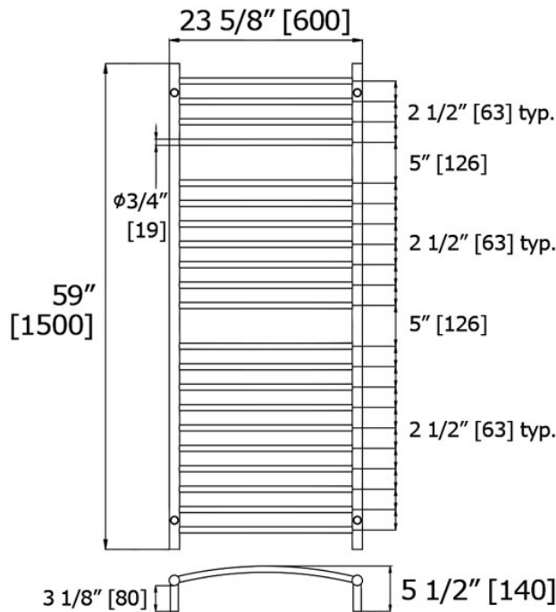
towel hanging space 21 1/4 [540mm]"
